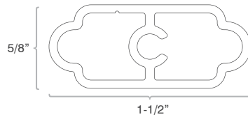
SCULPTURED PICKET actual size shown
